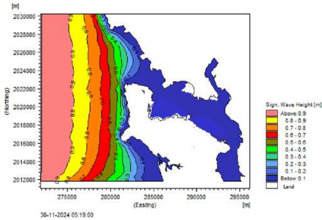
Figure 8: Spectral Wave Modelling: Existing and Proposed
