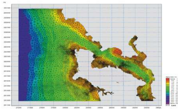
Figure 4: Bathymetry with mesh and boundary condition
