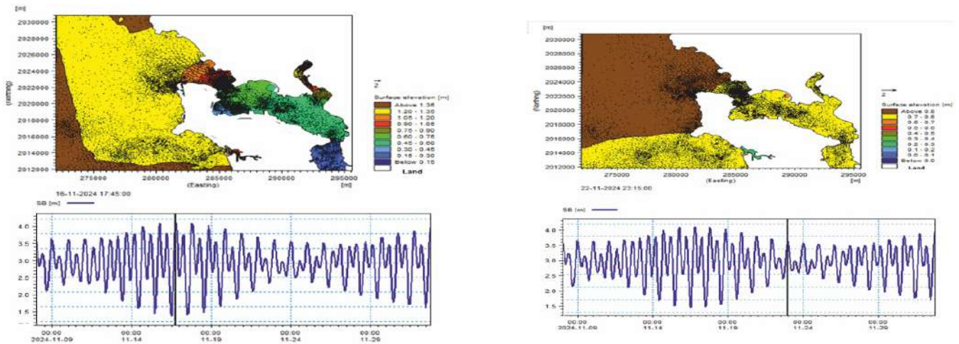
Figure 6: Results obtained for Hydrodynamic Model for Spring and Neap tide (Proposed)
