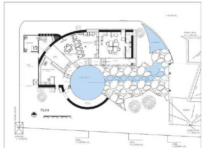
Figure 3- Bamboo Symphony, Bangalore centre line plan of roof and floor plan. (Source- Manasaram Architects)
