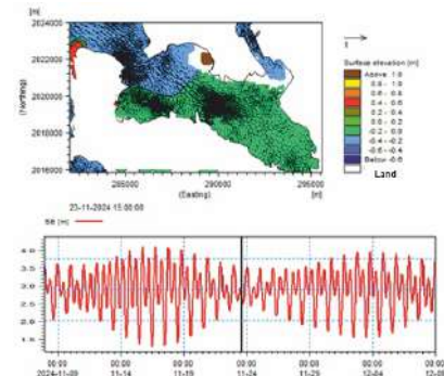
Figure 5: Results obtained for Hydrodynamic Model for Spring and neap tide (Existing)
