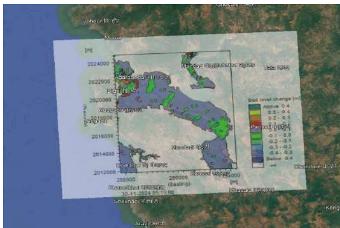
Figure 7: Results showing Sediment Transport at the end of simulation for proposed layout
