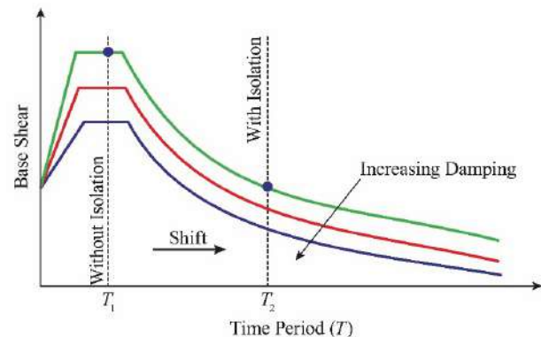
Figure 1. Effect of seismic isolation on base shear
