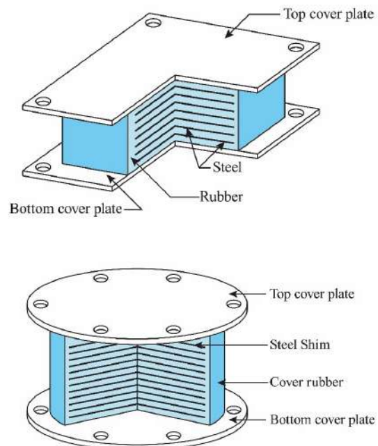
Figure 3. Square and Circular Elastomeric isolators
