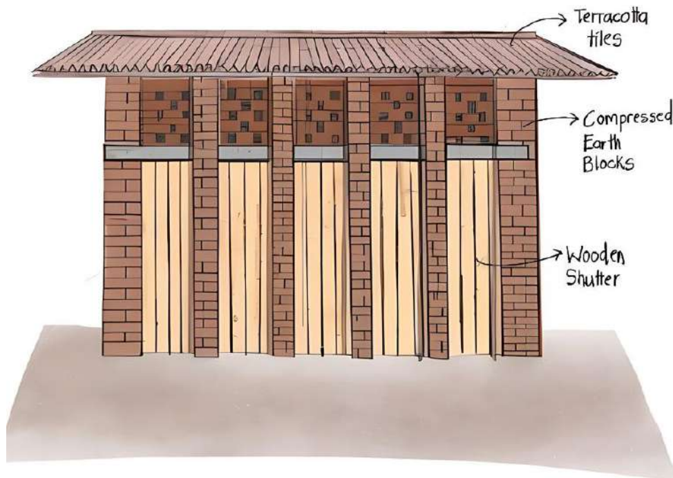
Figure 2-CSEB Composite Design (Source -Authors)
