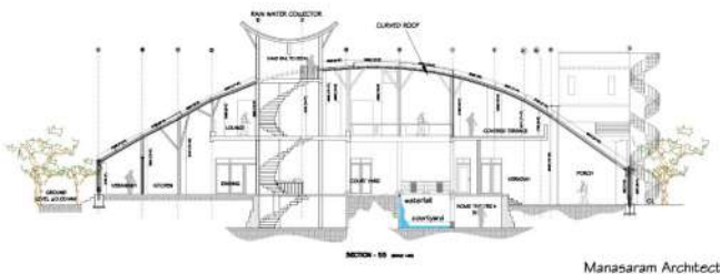
Figure 5- Section of house of five elements (Source -Manasaram Architects)
